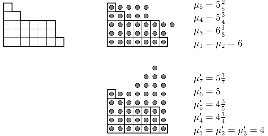
FIGURE 1. Calculating the slope of a monomial scheme.
