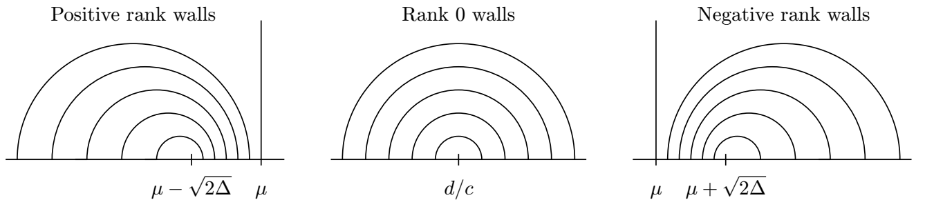
FIGURE 3. Relevant potential Bridgeland walls for (i) a positive rank object with \Delta \geq 0 ; (ii) a rank 0 object with Chern character cL + dL^2 and c \neq 0 ; (iii) a negative rank object with \Delta \geq 0 . For positive (resp. negative) rank walls, the centers of the walls converge to \mu - \sqrt{2\Delta} (resp. \mu + \sqrt{2\Delta} ).
