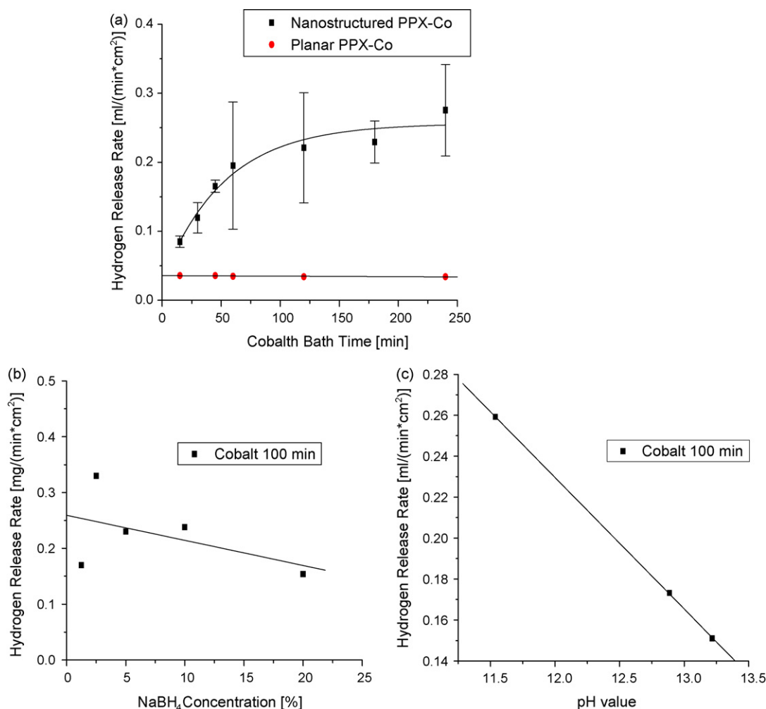
Fig. 4. (a) The hydrogen release rate (mL(min cm 2 ) -1 ) from the nanoporous and planar cobalt surface measured in 2.5% NaBH 4 and 1% NaOH at 25 °C. (b) Hydrogen release rate dependence on NaBH 4 concentration measured for a 100-min bath time sample at a pH of 11.5 and at 25 °C. (c) Hydrogen release rate dependence on pH measured for a 100-min bath time sample with 2.5% NaBH 4 concentration at 25 °C.
