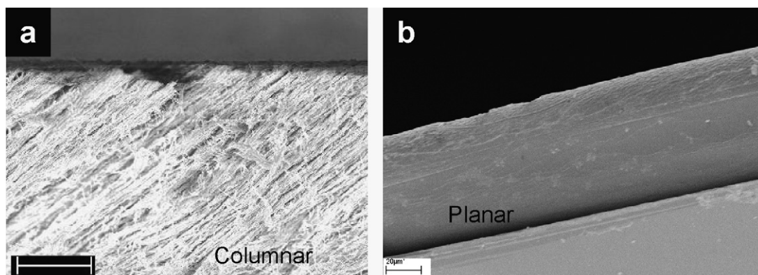
Fig. 1. Cross-sectional SEM images of PPX films deposited under (a) oblique angle (columnar morphology) and (b) conventional (bulk) methods (scale bar: 20 \mu\text{m} ).
