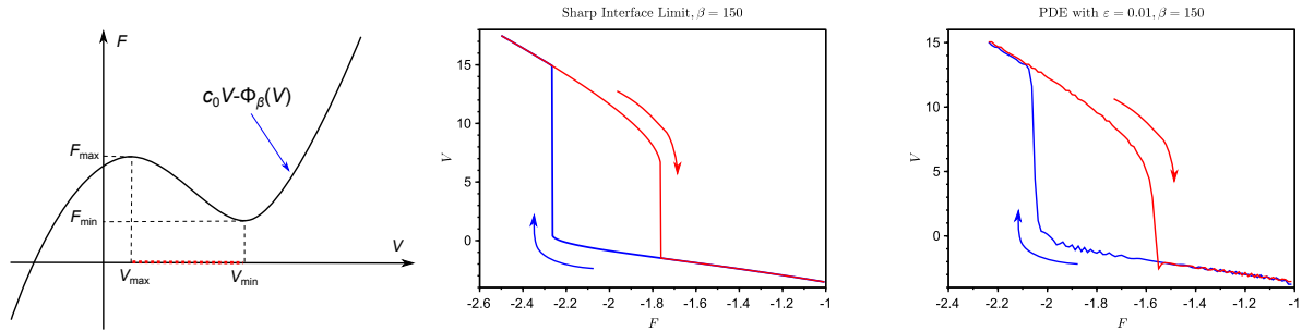
Figure 1: Hysteresis loop in the problem of cell motility. (Left) The sketch of the plot for c_0 V - \Phi_\beta(V) ; (Center,Right) Simulations of V = V(F) , (Center): solution of (10) (Right): solution of PDE system (17)-(18). On both figures (Center) and (Right) arrows show in what direction the system (V(t), F(t)) evolves as time t grows; blue curve is for F_\downarrow(t) , red curve is for F_\uparrow(t) .
