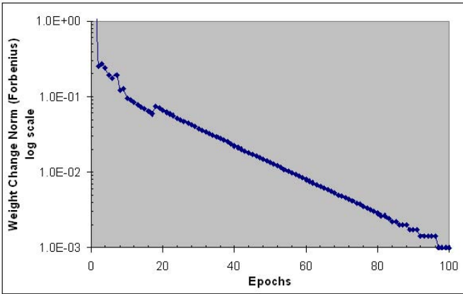
Fig. 6. Variation of Forbenius norm of the weight change matrix with no. of epochs
