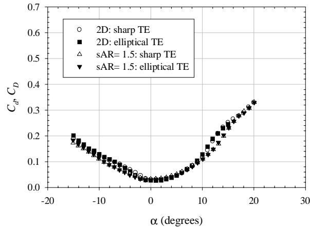
Figure 64: Trailing-edge geometry effect on drag coefficient at Re_c = 80,000 on cambered plates in the wind tunnel with UND-FBI
