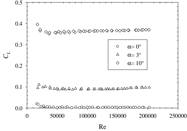
Figure 42: Lift coefficient variation with Re for AR = 1 flat-plate wing with UND-FB2
