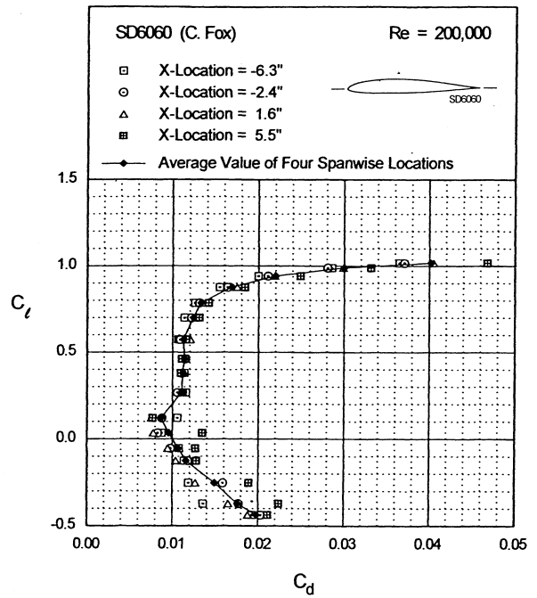
Figure 75: Drag polar for SD6060 airfoil at Re_c = 200,000 (Selig et al., 1995)
