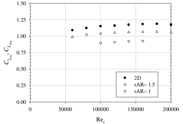
Figure 56: Maximum lift coefficient as a function of Re_c for cambered wings with UND-FBI
