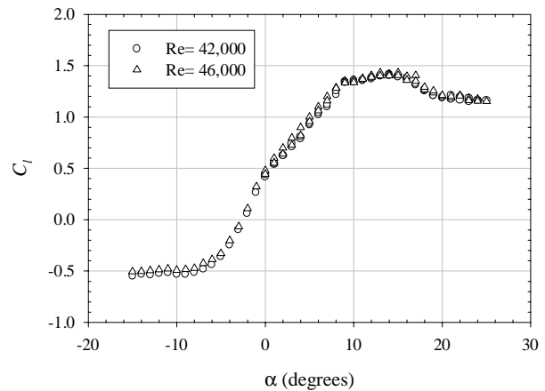
Figure 27: 2D lift coefficient on the Eppler 61 airfoil in the water tunnel with UND-FB2
