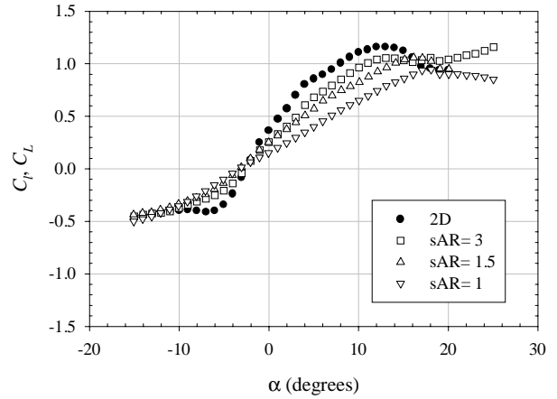
Figure 52: Lift coefficient on cambered plates at Re_c = 140,000 with UND-FBI
