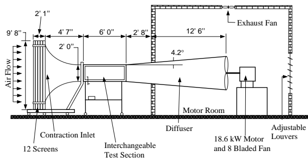
Figure 9: Schematic of the low-speed wind tunnel
