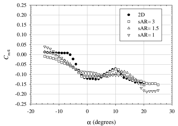
Figure 54: Pitching moment coefficient on cambered plates at Re_c = 140,000 with UND-FBI
