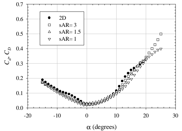
Figure 53: Drag coefficient on cambered plates at Re_c = 140,000 with UND-FBI
