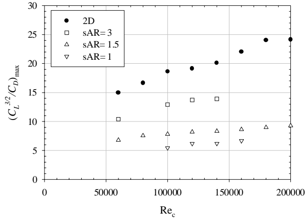
Figure 59: Maximum C_L^{3/2}/C_D ratio as a function of Re_c for cambered wings with UND-FBI
