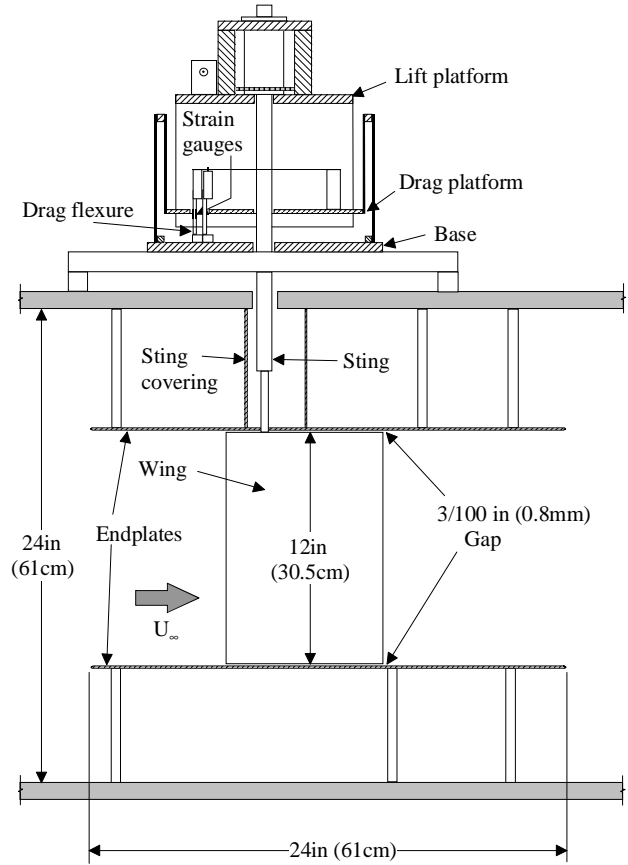
Figure 11: UND-FB1 balance arrangement (1) with two endplates in the wind tunnel
