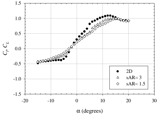
Figure 49: Lift coefficient on cambered plates at Re_c = 60,000 with UND-FBI
