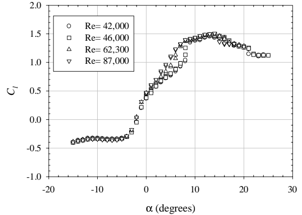
Figure 24: 2D lift coefficient on the Eppler 61 airfoil in the wind tunnel with UND-FB2
