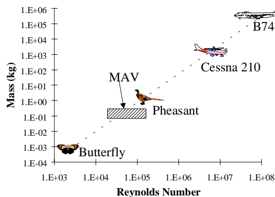
Figure 1: Reynolds number range for flight vehicles
