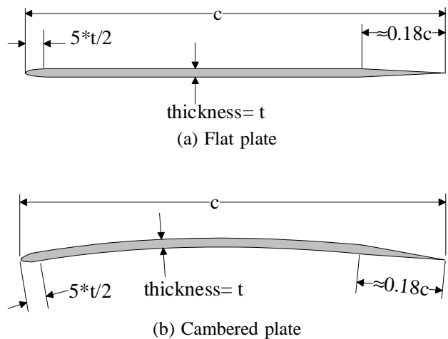
Figure 12: Airfoil geometry for models with tapered trailing edge
