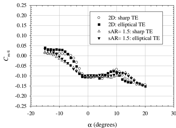
Figure 65: Trailing-edge geometry effect on pitching moment coefficient at Re_c = 80,000 on cambered plates in the wind tunnel with UND-FBI
