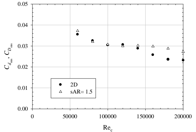
Figure 57: Minimum drag coefficient as a function of Re_c for cambered wings with UND-FBI
