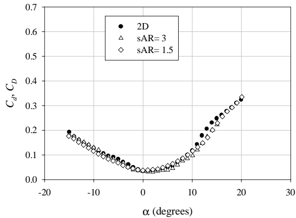
Figure 50: Drag coefficient on cambered plates at Re_c = 60,000 with UND-FBI
