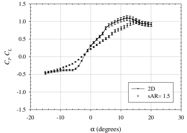
Figure 13: Uncertainties in lift coefficient for cambered plates at Re_c = 60,000 with UND-FB1
