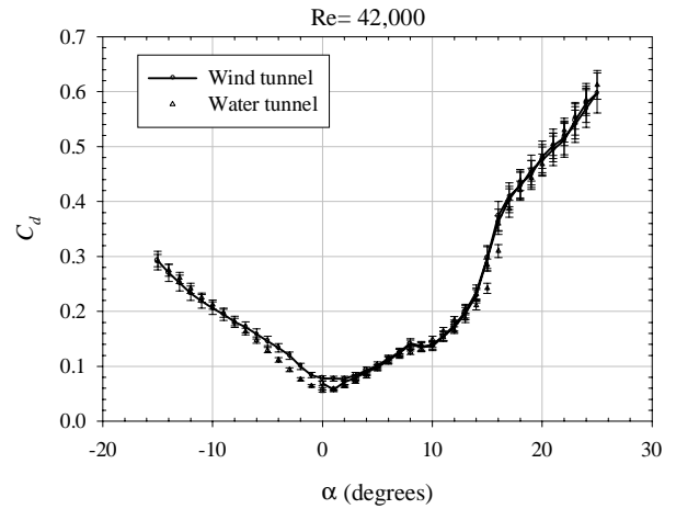
Figure 33: Comparison of the 2D drag coefficient on the Eppler 61 airfoil in wind and water tunnels with UND-FB2
