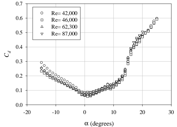
Figure 25: 2D drag coefficient on the Eppler 61 airfoil in the wind tunnel with UND-FB2
