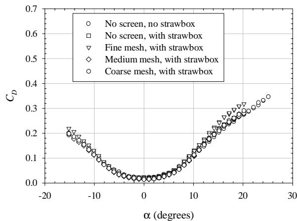
Figure 67: Freestream turbulence effect on drag coefficient at Re_c = 60,000 in the wind tunnel for the sAR = 1.5 flat-plate model with UND-FBI
