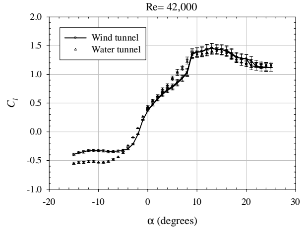
Figure 32: Comparison of the 2D lift coefficient on the Eppler 61 airfoil in wind and water tunnels with UND-FB2
