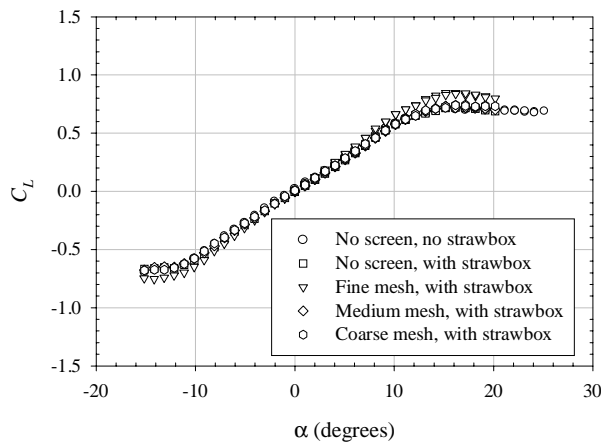
Figure 66: Freestream turbulence effect on lift coefficient at Re_c = 60,000 in the wind tunnel for the sAR = 1.5 flat-plate model with UND-FBI
