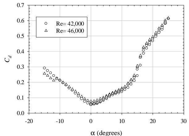
Figure 28: 2D drag coefficient on the Eppler 61 airfoil in the water tunnel with UND-FB2
