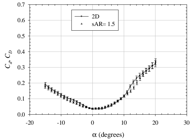
Figure 14: Uncertainties in drag coefficient for cambered plates at Re_c = 60,000 with UND-FB1
