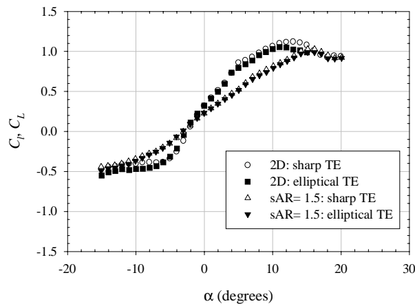
Figure 63: Trailing-edge geometry effect on lift coefficient at Re_c = 80,000 on cambered plates in the wind tunnel with UND-FBI
