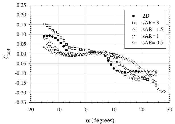
Figure 39: Pitching moment coefficient on flat plates at Re_c = 140,000 with UND-FBI
