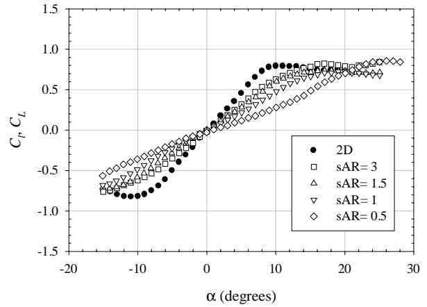
Figure 37: Lift coefficient on flat plates at Re_c = 140,000 with UND-FBI
