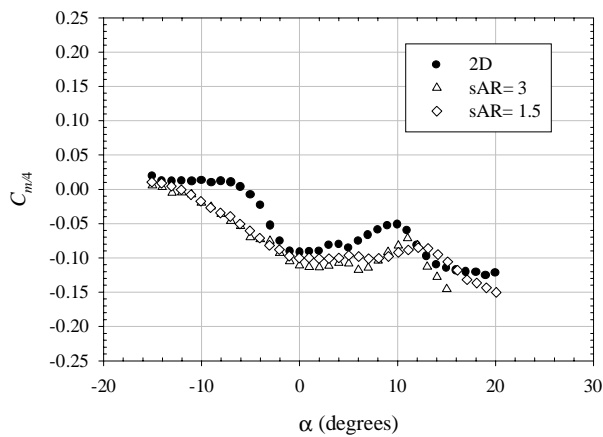
Figure 51: Pitching moment coefficient on cambered plates at Re_c = 60,000 with UND-FBI
