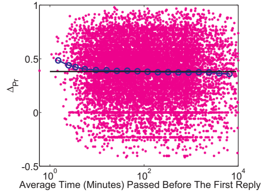
Fig. 10. Sentiment Change Indicator ( \Delta_{Pr} ) vs. the time elapsed before the first reply
