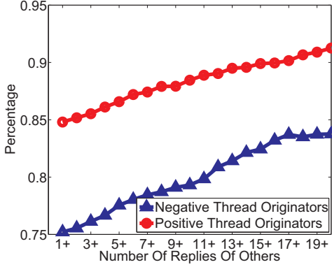
Fig. 5. Circle: y = p(S_1 = + | S_0 = +, n_1 \geq x) ; Triangle: y = p(S_1 = + | S_0 = -, n_1 \geq x) , where n_1 is the number of replies from people other than the thread originator, S_0 and S_1 are initial-sentiment and subsequent-sentiment , respectively
