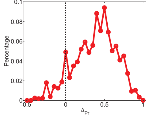
Fig. 7. Distribution of Sentiment Change Indicator ( \Delta_{Pr} ).
