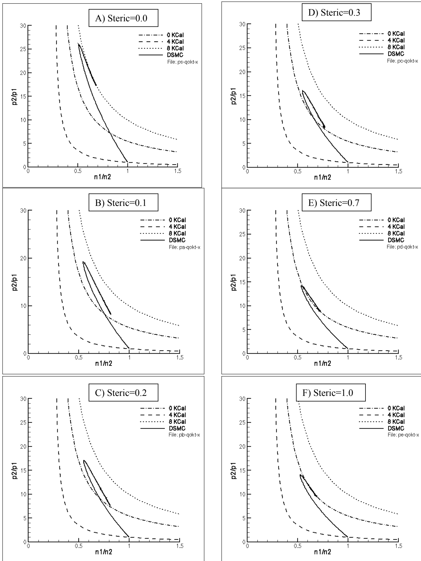
Figure 2. Rankine-Hugoniot plots for 8 kcal/mol exothermic and -4 kcal/mol endothermic reactions for various steric factors: (A) 0.0, (B) 0.1, (C) 0.2, (D) 0.3, (E) 0.7, (F) 1.0.
