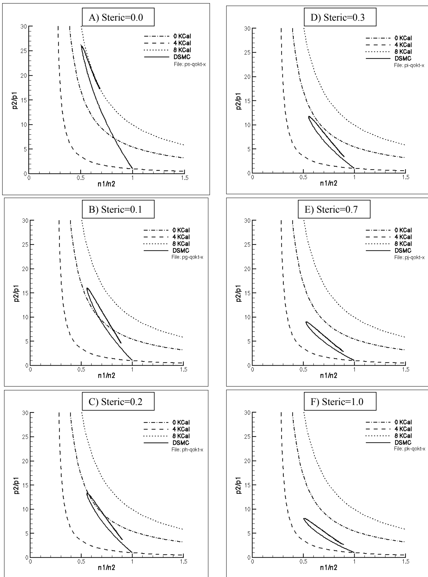
Figure 3. Rankine-Hugoniot plots for 8 kcal/mol exothermic and -8 kcal/mol endothermic reactions for various steric factors: (A) 0.0, (B) 0.1, (C) 0.2, (D) 0.3, (E) 0.7, (F) 1.0.
