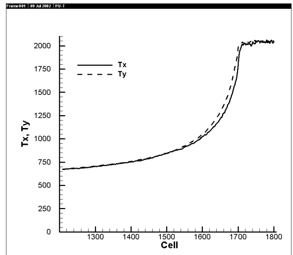
Figure 8. Rankine-Hugoniot plot and temperature results for steric factor = 0.0 ( -4 kcal/mol exothermic)
