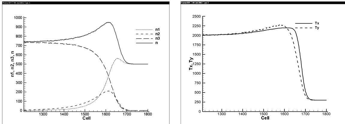
Figure 5. Species concentration and temperature results for steric factor = 1.0 ( 8 kcal/mol exothermic and -4 kcal/mol endothermic reactions)
