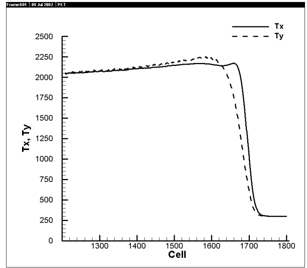
Figure 7. Rankine-Hugoniot plot and temperature results for steric factor = 0.0 ( 4 kcal/mol exothermic)
