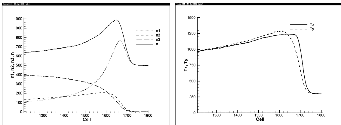
Figure 6. Species concentration and temperature results for steric factor = 1.0 ( 8 kcal/mol exothermic and -8 kcal/mol endothermic reactions)
