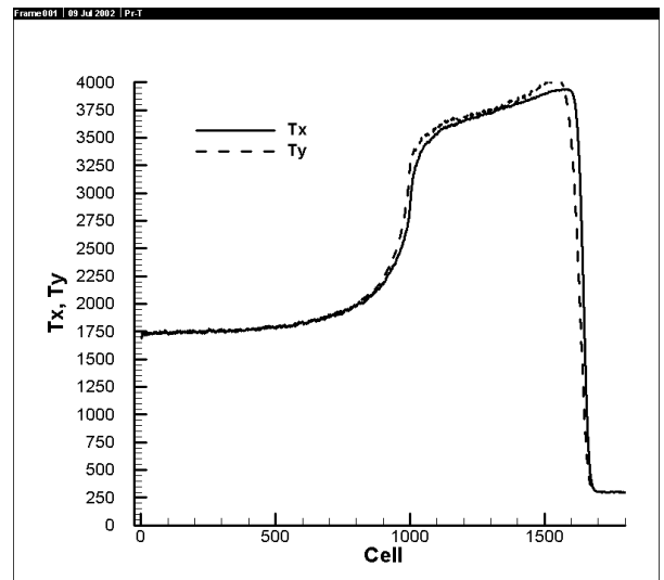
Figure 9. Species concentration and temperature results for steric factor = 1.0 ( 8 kcal/mol exothermic and 4 kcal/mol endothermic, with a spatial delay)
