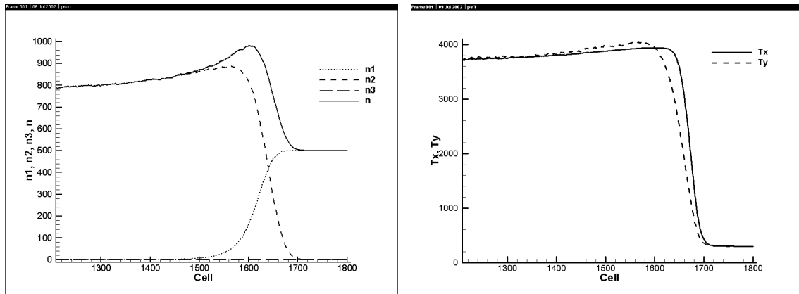
Figure 4. Species concentration and temperature results for steric factor = 0.0 ( 8 kcal/mol exothermic)
