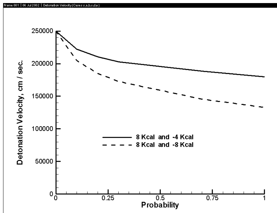
FIGURE 1. Detonation velocity vs. steric factor (probability) for two different endothermic reactions .
