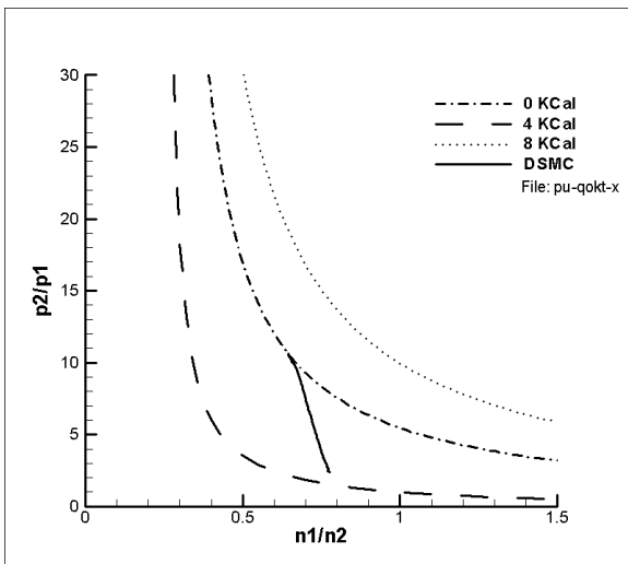
Figure 8. Rankine-Hugoniot plot and temperature results for steric factor = 0.0 ( -4 kcal/mol exothermic)
