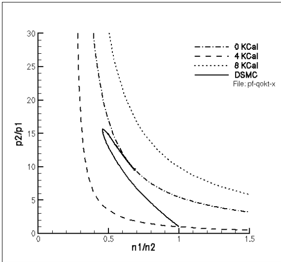
Figure 7. Rankine-Hugoniot plot and temperature results for steric factor = 0.0 ( 4 kcal/mol exothermic)
