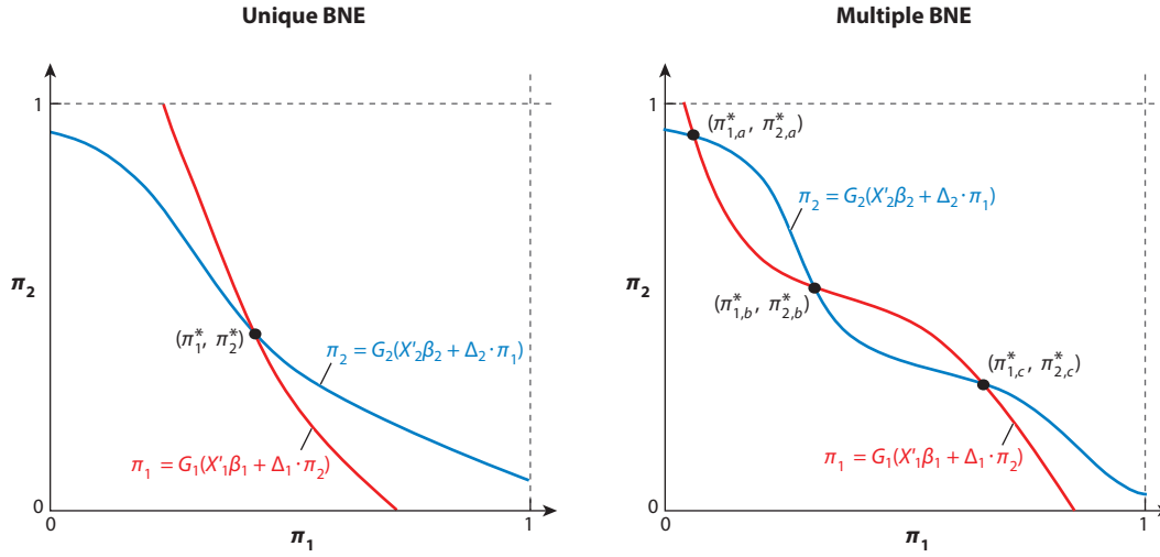
Figure 3 An illustration of Bayesian Nash equilibria (BNE).
