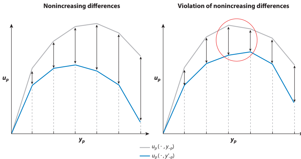
Figure 5 Nonincreasing differences. The red circle illustrates a violation of nonincreasing differences.
