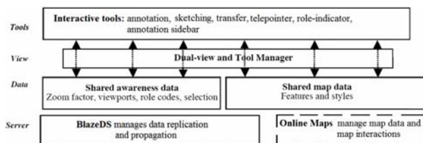
Figure 2. Prototype Architecture
